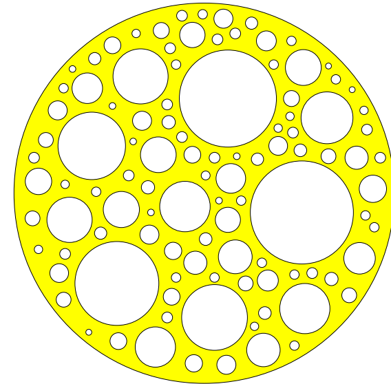
A Swiss cheese set with non-overlapping holes
